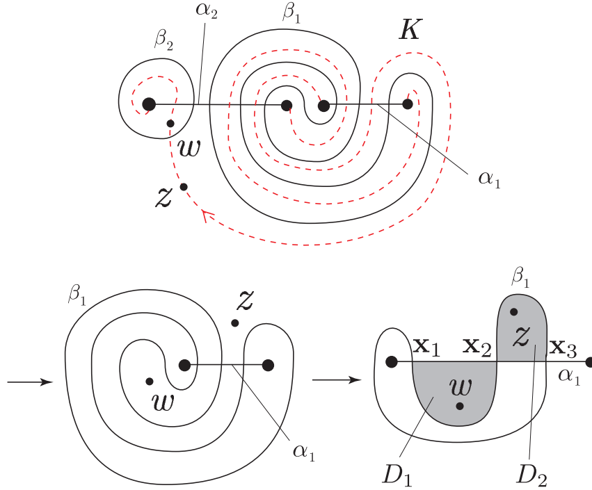
Figure 2: A double pointed Heegaard diagram of the trefoil knot and a move.
