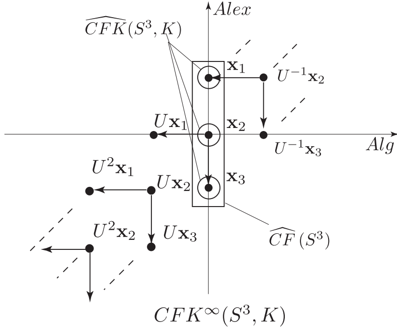
Figure 3: Differentials of CFK^\infty(S^3, K) and \widehat{CFK}(S^3, K) in it.
