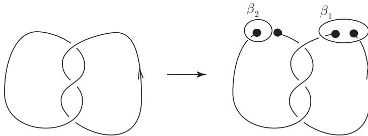
Figure 1: The trefoil knot and the Heegaard decomposition of S^3 .
